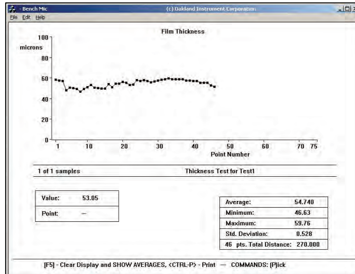
The Model DAQ-MIC Main Screen Showing Thickness Profile
