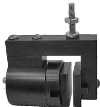
MT Series Small Air Grip for Film and Sheet with 25 mm x 25 mm (1 inch x 1 inch) Rubberized Inserts installed.
